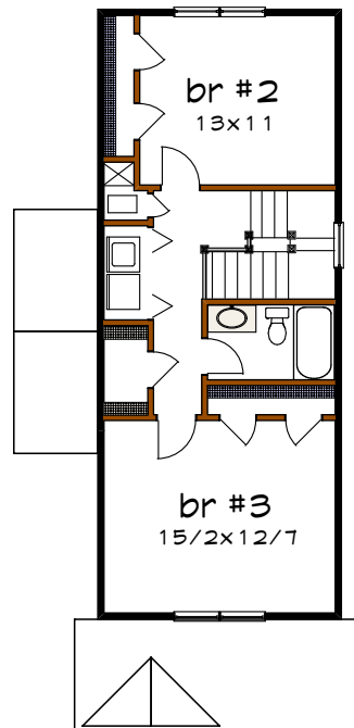
Floor 2 plan
