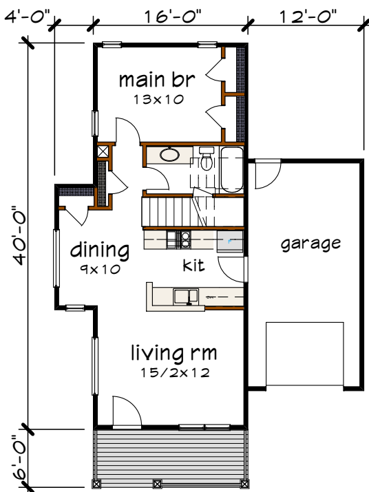
Floor 1 plan
