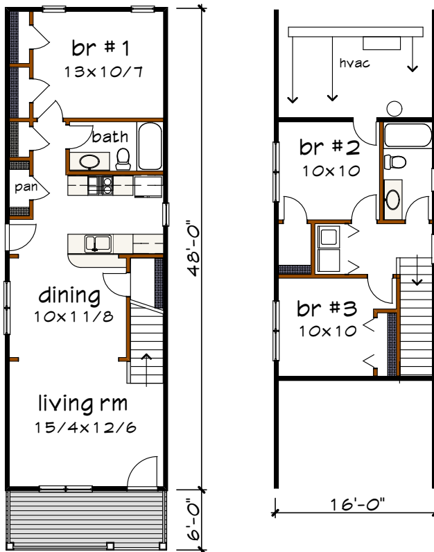
Floor 1 plan Floor 2 plan
