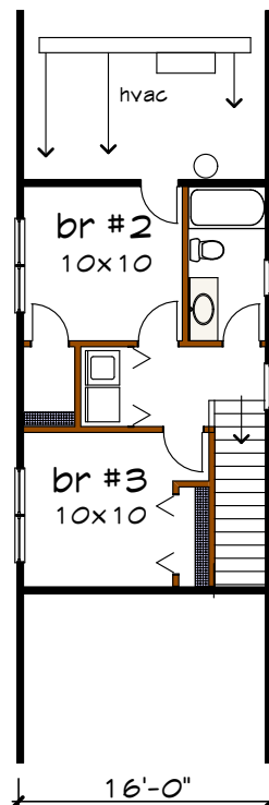
Floor 2 plan
