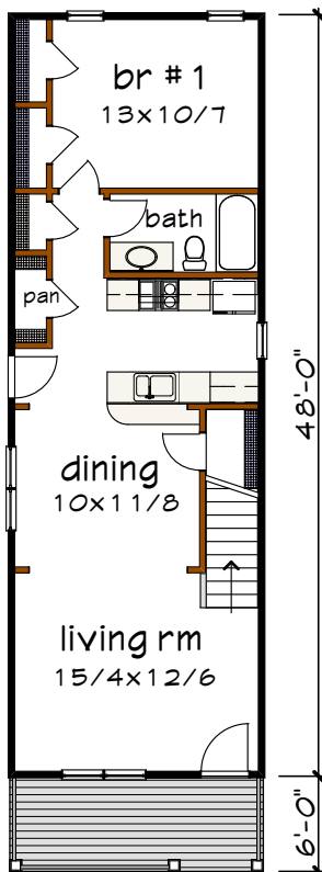
Floor 1 plan
