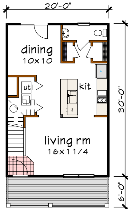
Floor 1 plan
