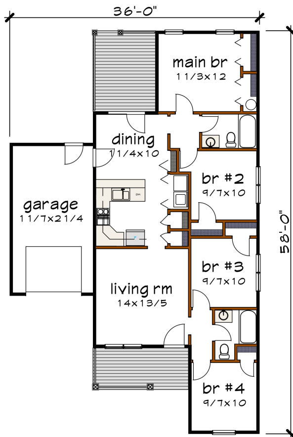
Floor 1 plan
