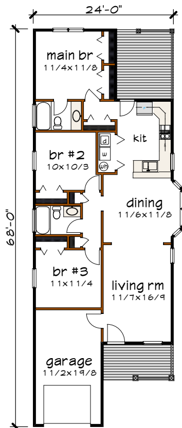
Floor 1 plan
