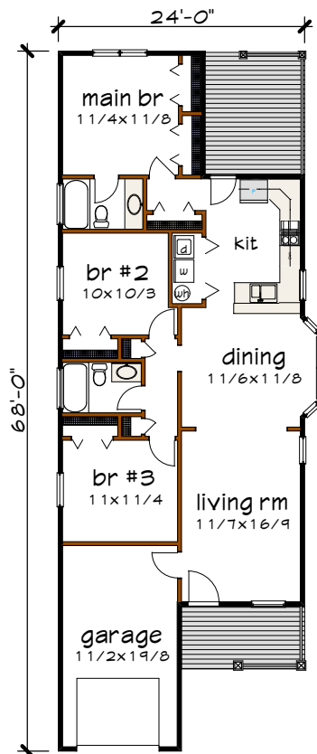
Floor 1 plan
