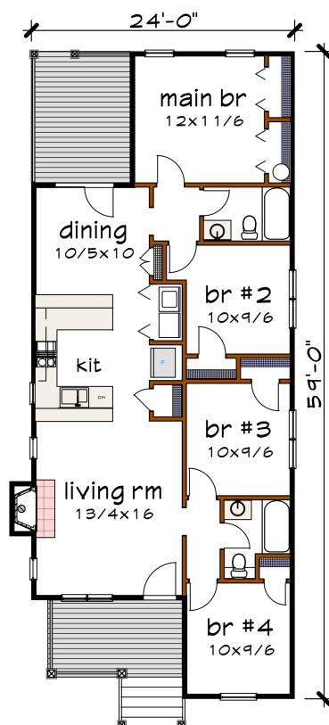
Floor plan
