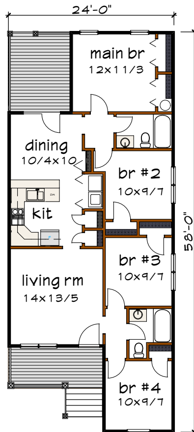
Floor 1 plan
