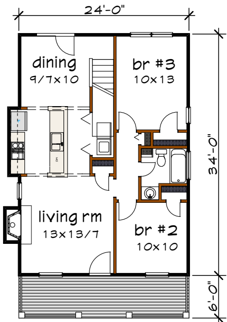
Floor 1 plan
