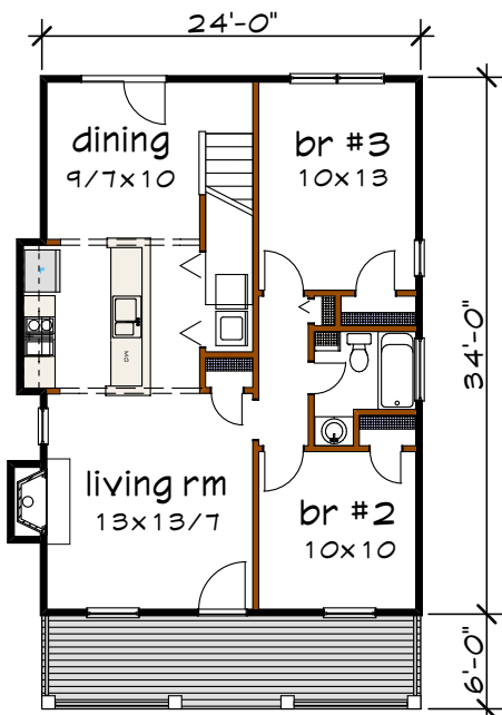
Floor 1 plan
