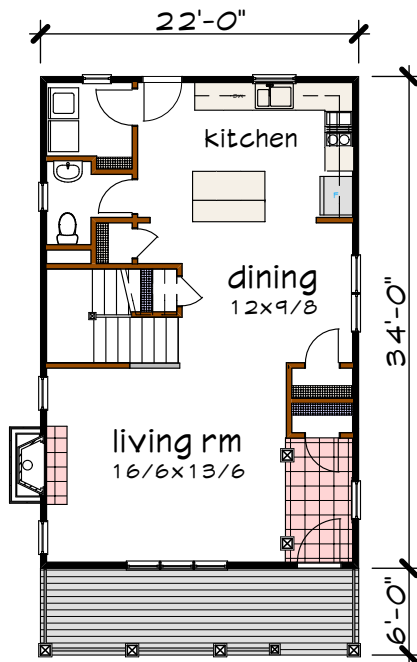
Floor 1 plan
