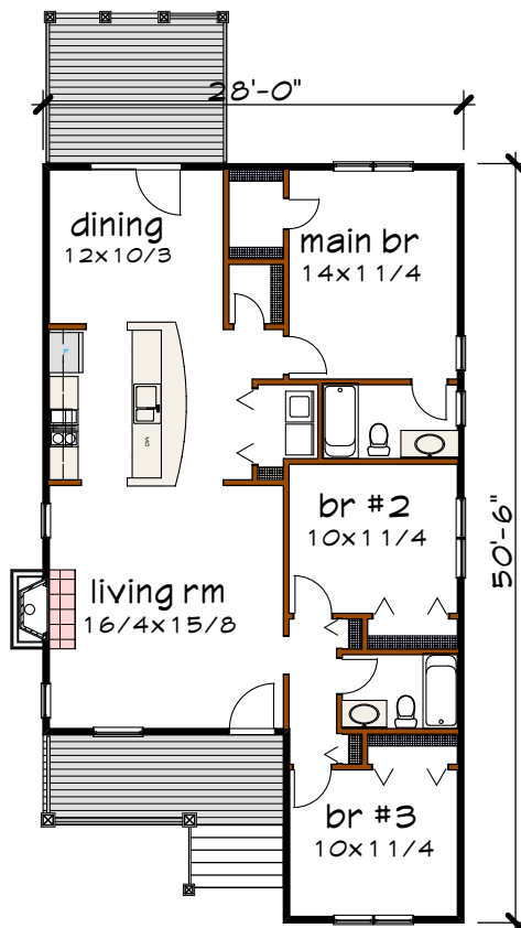
Floor Plan
