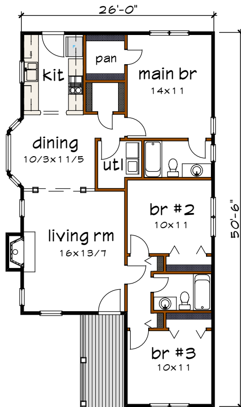
Floor 1 plan
