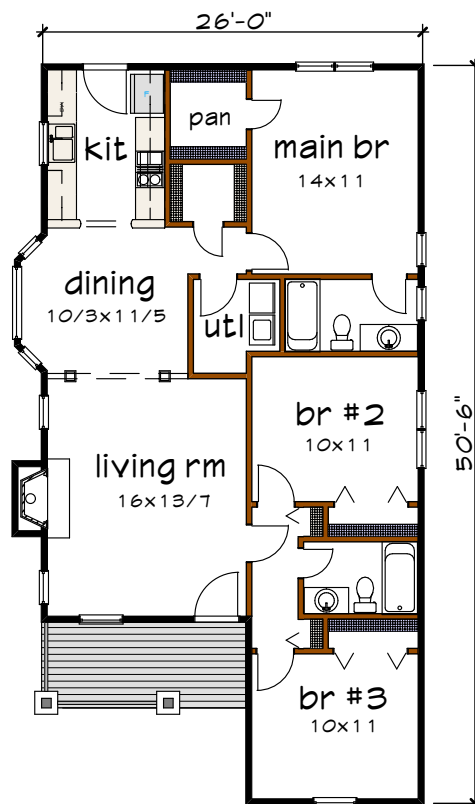
Floor 1 plan
