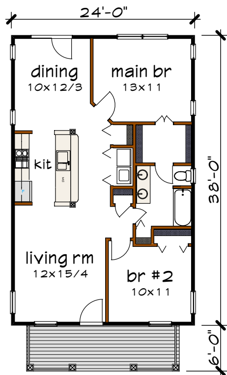
Floor 1 plan
