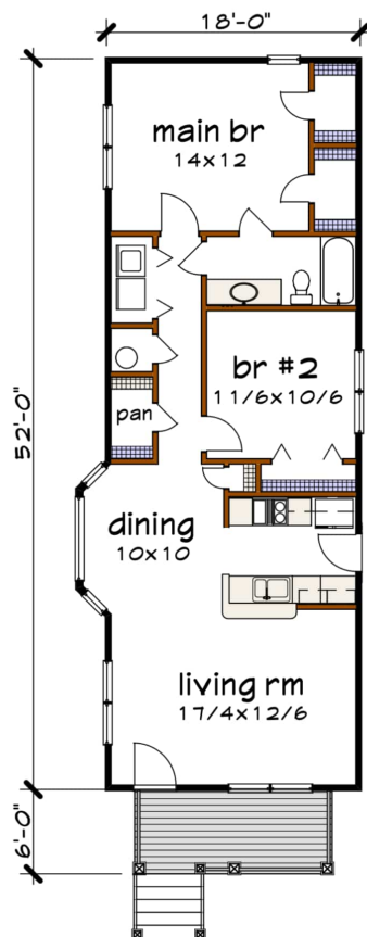
Floor 1 plan
