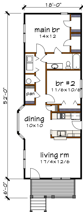
Floor 1 plan
