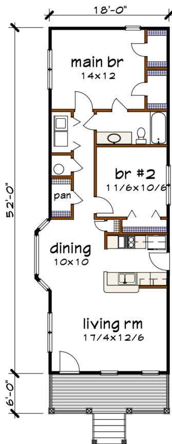
Floor 1 plan
