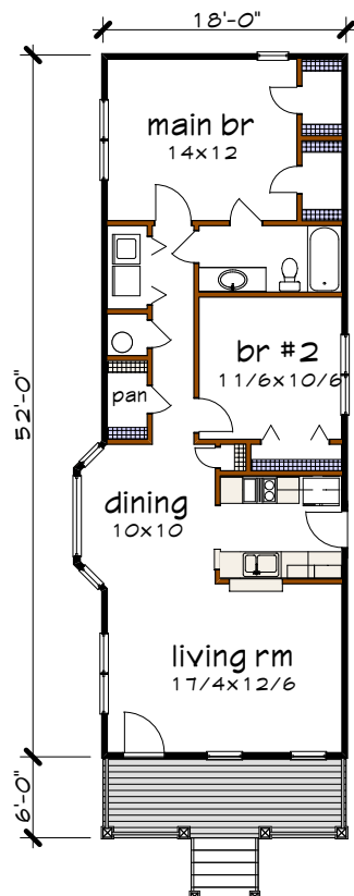
Floor 1 plan
