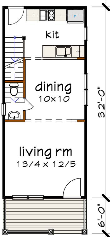
Floor 1 plan
