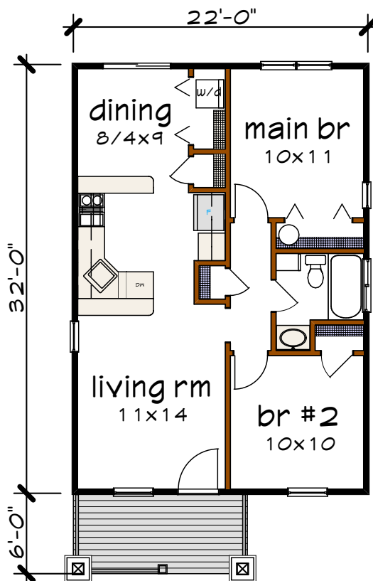
Floor 1 plan
