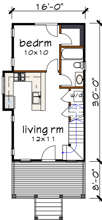
Floor 1 plan
