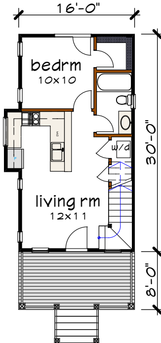
Floor 1 plan
