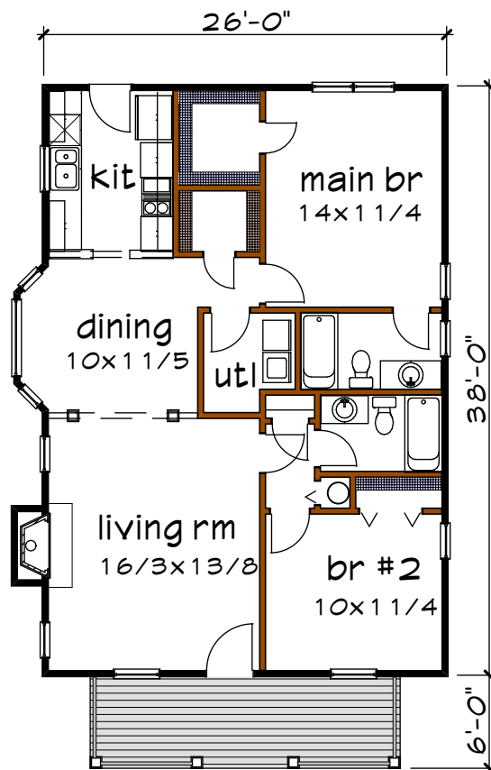
Floor 1 plan
