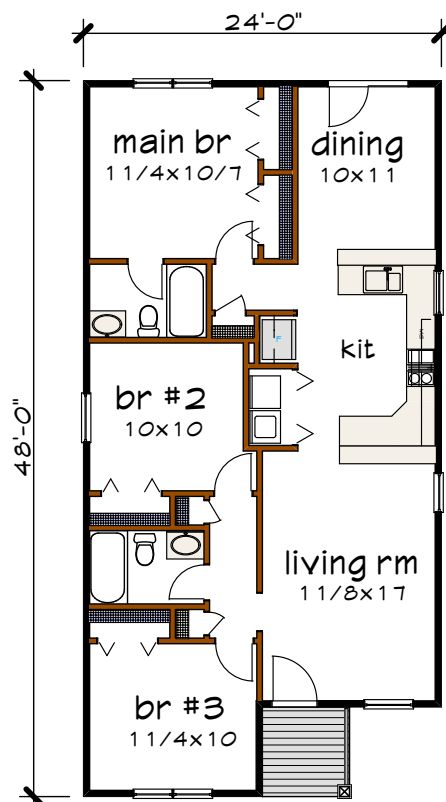
Floor Plan
