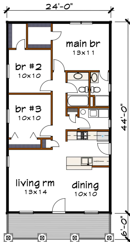
Floor 1 plan
