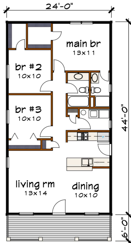
Floor 1 plan
