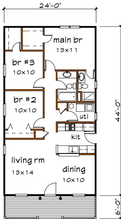
Floor 1 plan
