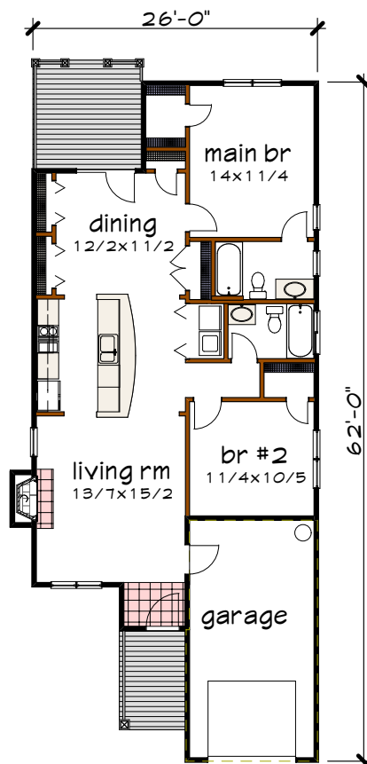
Floor 1 plan
