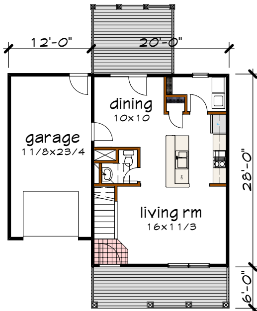
Floor 1 plan
