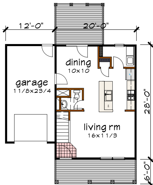
Floor 1 plan
