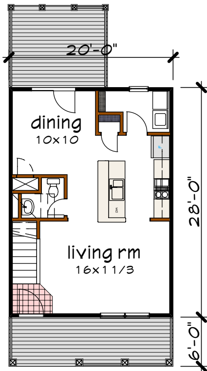
Floor 1 plan
