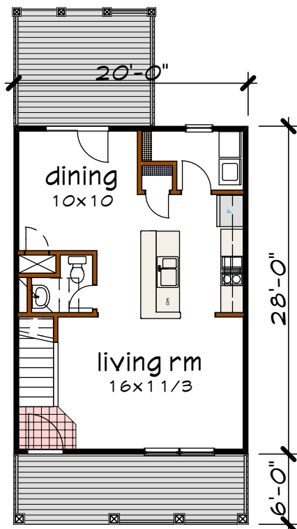
Floor 1 plan
