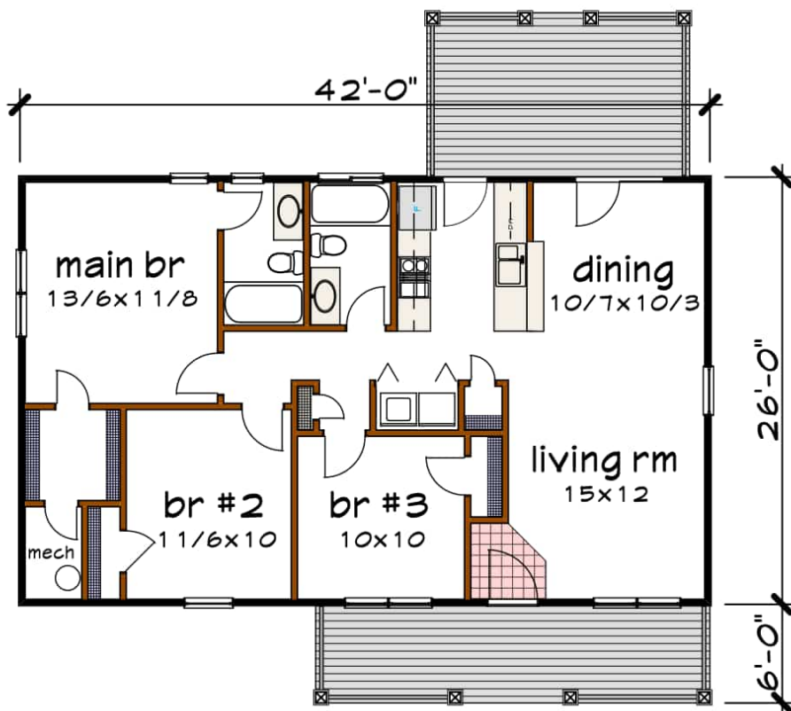
Floor 1 plan
