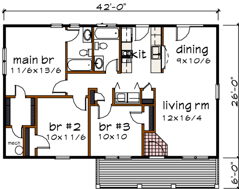
Floor 1 plan
