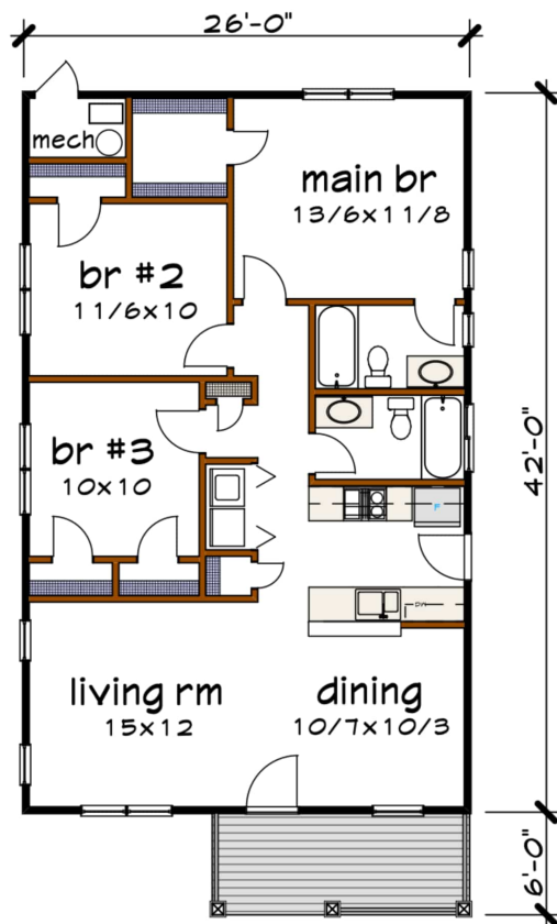
Floor 1 plan
