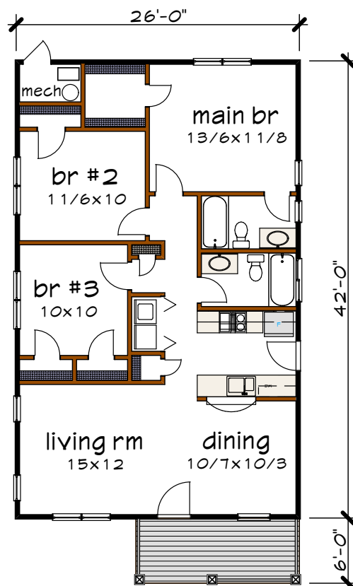
Floor 1 plan
