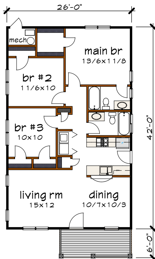
Floor 1 plan
