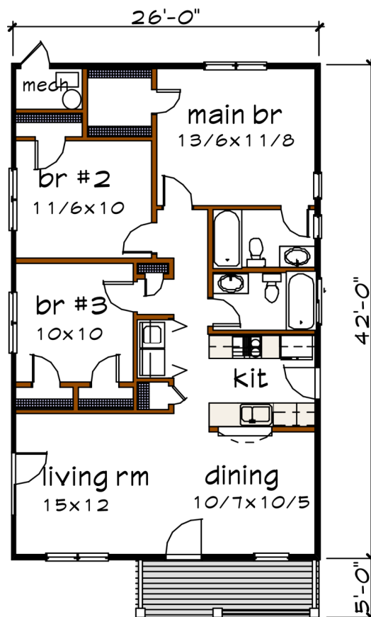
Floor 1 plan
