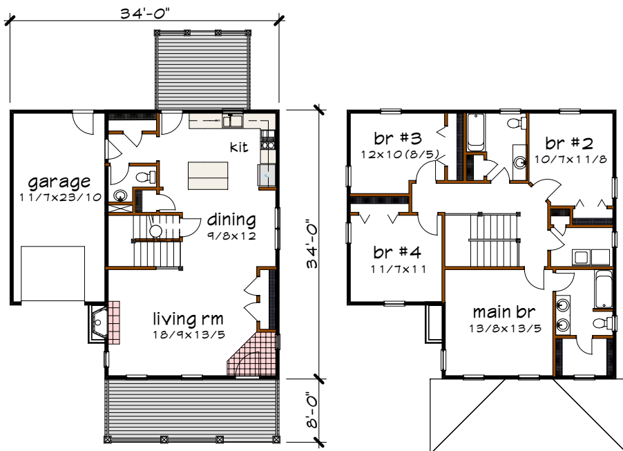
Floor 1 plan
