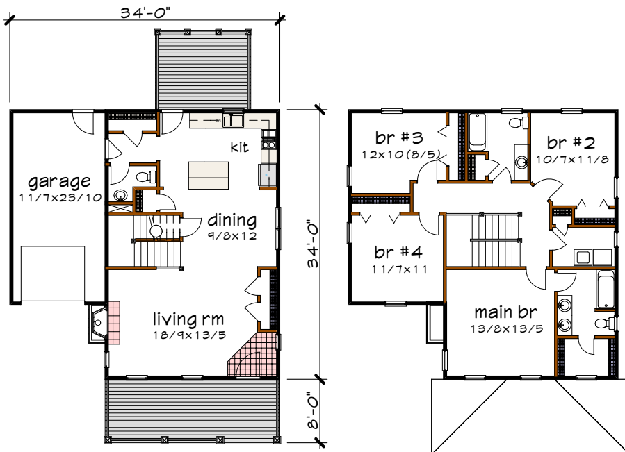
Floor 1 plan
