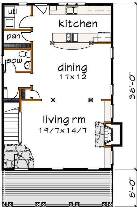
Floor 1 plan
