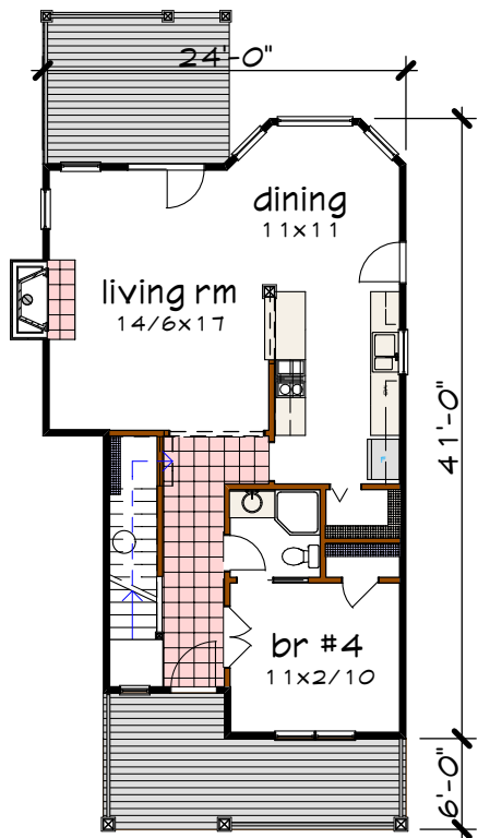
Floor 1 plan
