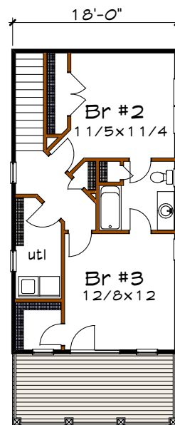
Floor 2 plan
