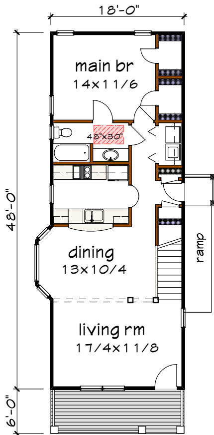
Floor 1 plan
