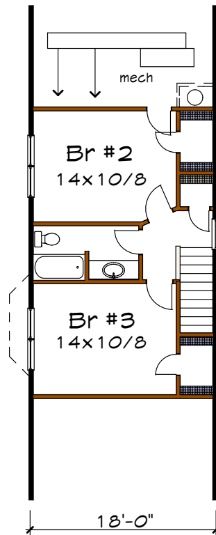
Floor 2 plan
