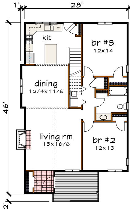
Floor 1 plan
