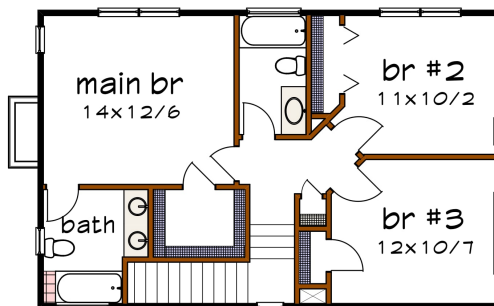
Floor 2 plan
