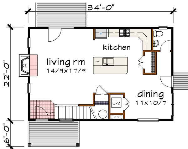
Floor 1 plan
