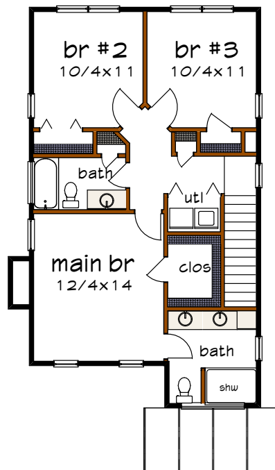
Floor 2 plan
