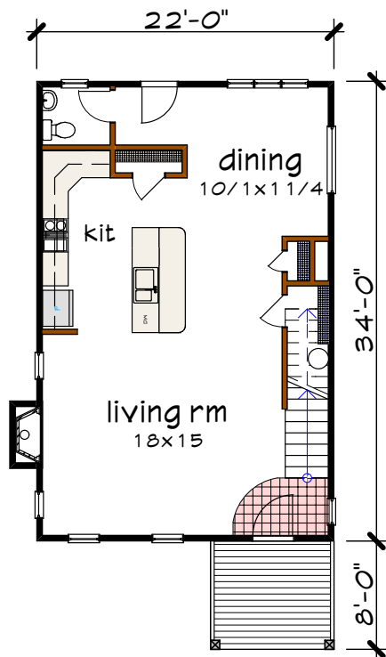
Floor 1 plan
