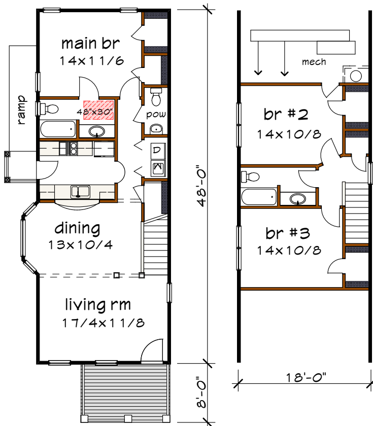
Floor 1 plan
